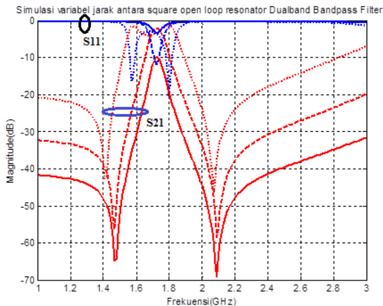
Gambar 10: Simulasi variabel jarak antar square open loop resonator , s (dotted line: s = 0,1 mm, dash line: s = 0,6 mm dan solid line s = 1,1 mm).
