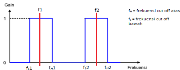
Gambar 1: Respon Dual-Band Band Pass Filter ideal.
