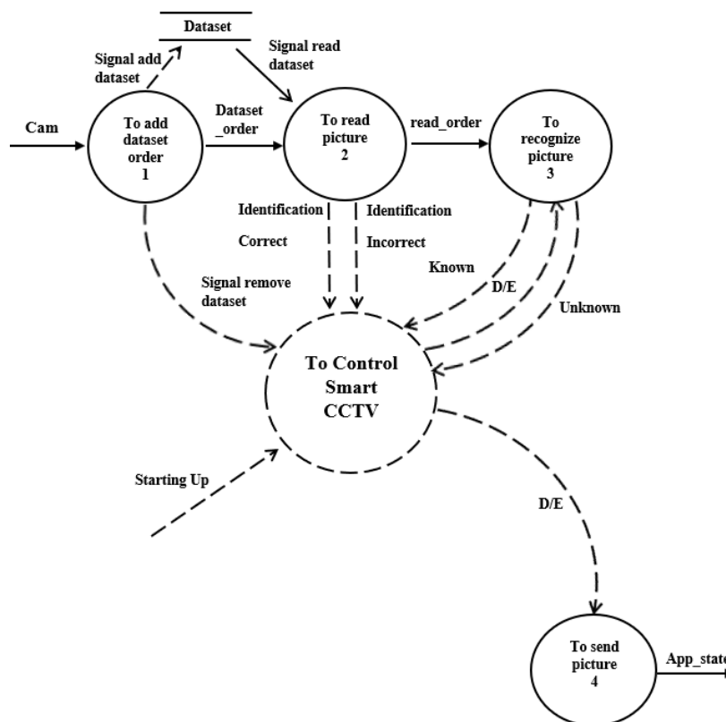
Gambar 6. DFD/CFD level 1 "smart cctv"
