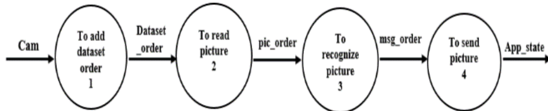
Gambar 5. DFD Level 1 "smart cctv"
