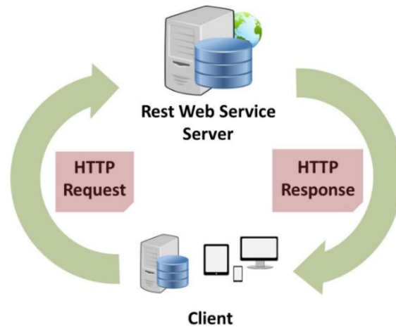
Figure 5. REST architecture [12].
