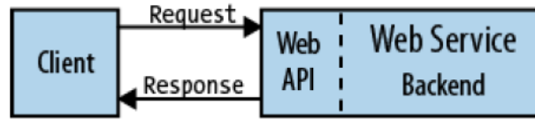
Figure 2. Web API [11]
