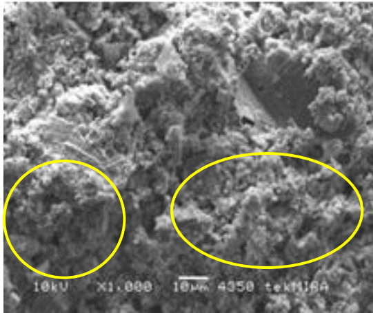
Fig. 4. SEM Images of FA-10 (Magnification 1000X). Yellow circle marks the tobermorite formation
