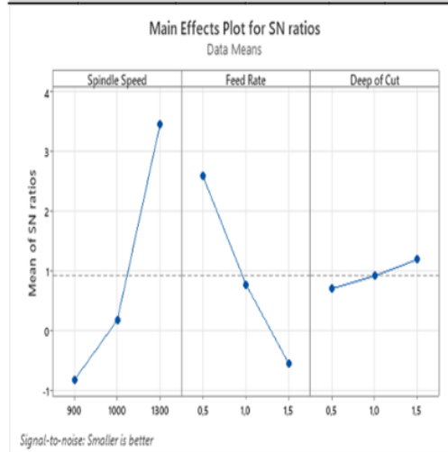
Fig. 5. Means surface roughness ratio S/N
