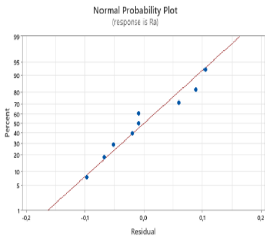
Fig. 6. Normalized probability plot of the residuals for surface roughness
