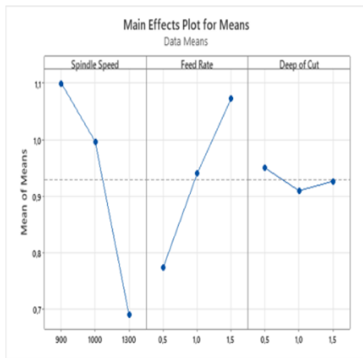
Fig. 4. The Influence of Machining Processes on Surface Roughness
