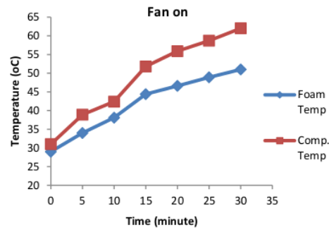
Figure 10. Temperature of inner enclosure with fan on condition
