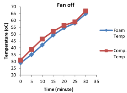
Figure 9. Temperature of inner enclosure with fan off condition
