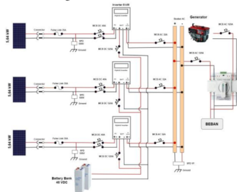
Fig. 3. Hybrid Power Plant System Wiring
