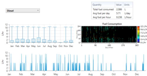
Fig. 2. Fuel Consumption
