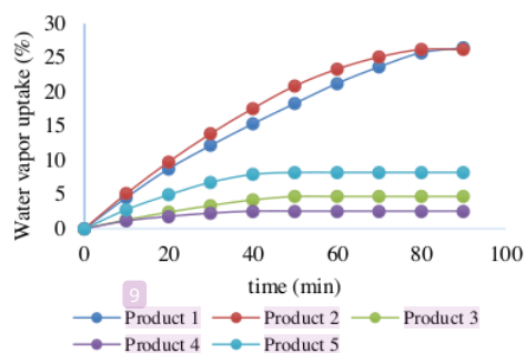
Fig. 2. Water vapor uptake of chitosan/PVA film products
