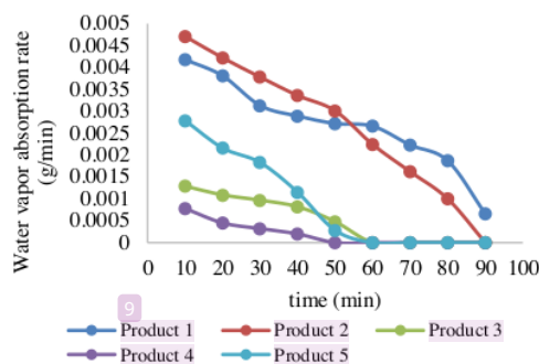
Fig. 3. Water vapor absorption rate of chitosan/PVA films
