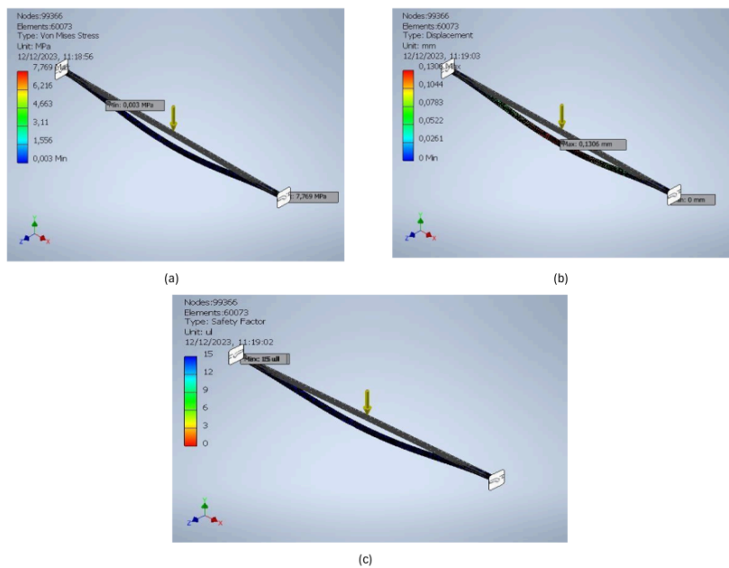
Figure 8. Simulation results from Autodesk Inventor; (a) Von Mises Stress; (b) Displacements; (c) Safety Factor
