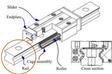
Figure 3. Structure of the linear guide rail
