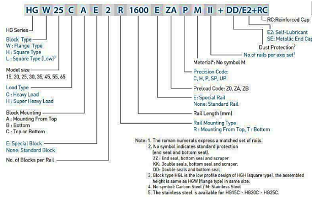
Figure 5. Linear guide rail serial code/symbol indication
