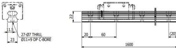
Figure 4. Dimensions of the guide rail
