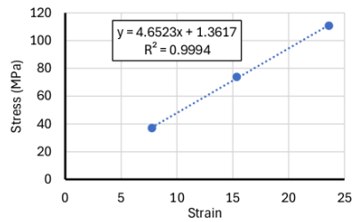
Figure 10. Linear regression plot
