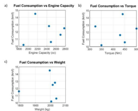
Fig 3.1 Relationship between fuel consumption vs engine capacity (a), fuel consumption vs torque (b), fuel consumption vs weight (c)
