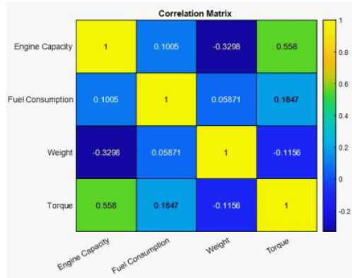
Fig. 3.5 explains the correlation between the variables studied, namely engine capacity, fuel consumption, vehicle weight and torque
