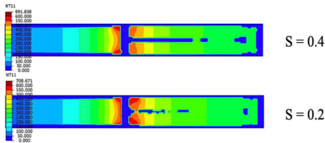
Figure 13. Effect of tool density on peak temperature.
