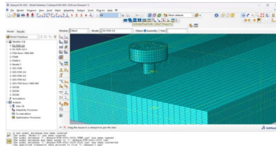
Figure 4. Tool and plate assembled from the top view.
