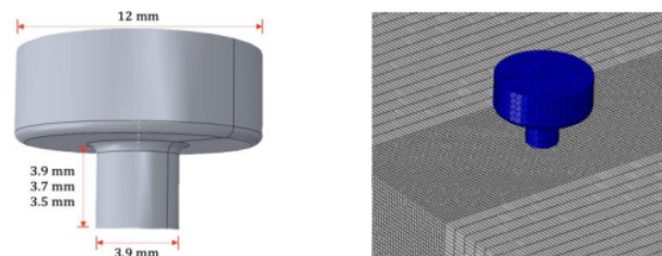
Figure 7. (left) Fabrication Model of the Chisel/Tool Used in the Initial Simulative Experiment (Model-1), (right) Its Net Boundary Near the Weld.
