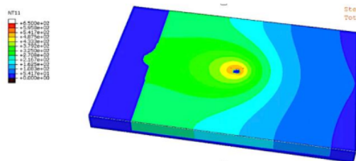
Figure 9. Visual simulation of sources and heat propagation that occur during the welding process.
