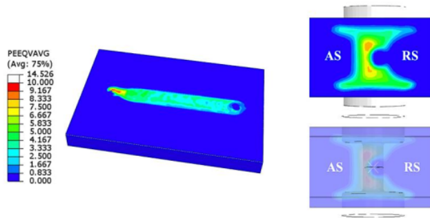
Figure 12. Range and scope of plastic strains.
