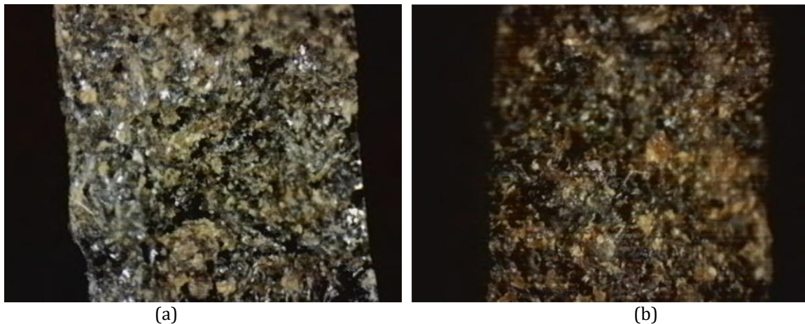
Figure 5. Fracture-surface morphology at 50× magnification: (a) representative high-tensile-strength specimen showing a relatively dense, resin-rich surface and (b) representative low-tensile-strength specimen showing a more porous, wood-particle-dominated surface with evidence of particle pull-out.
