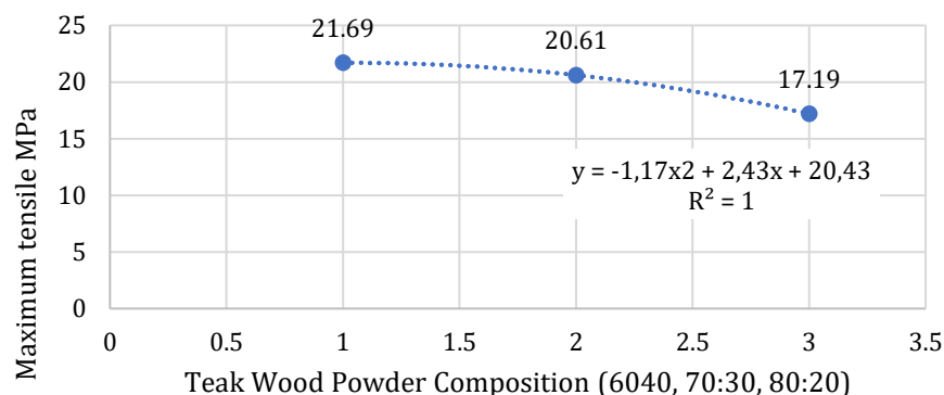
Figure 7. Effect of teak wood powder–epoxy composition on mean tensile strength averaged across hot-pressing temperatures.
