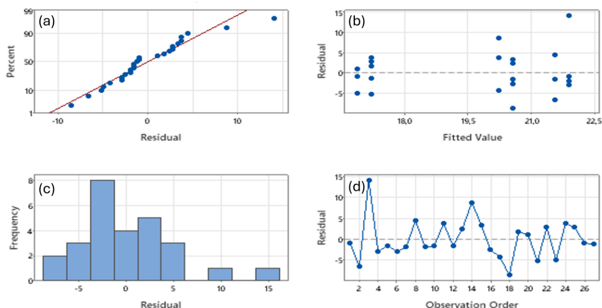
Figure 6. Residual diagnostics for the ANOVA model: (a) normal probability plot, (b) residuals versus fitted values, (c) residual histogram, and (d) residuals versus observation order.
