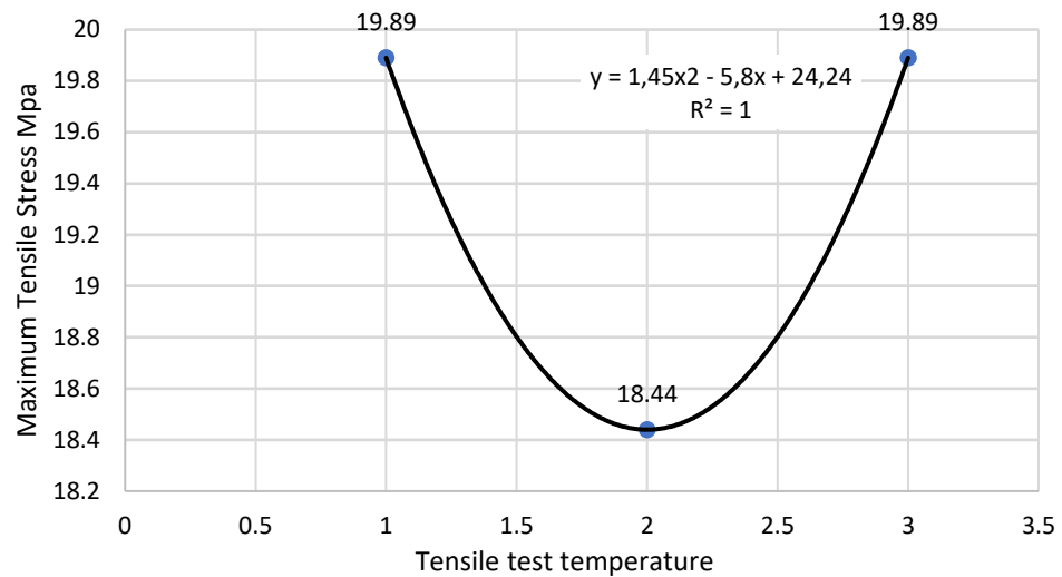
Figure 8. Effect of hot-pressing temperature on mean tensile strength averaged across composite compositions.
