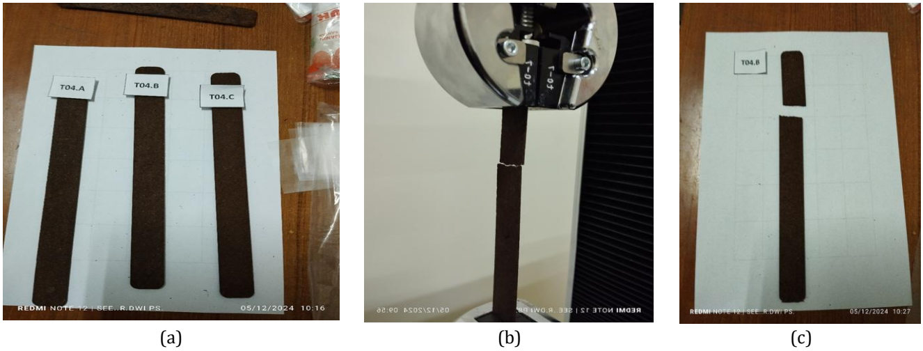
Figure 4. Tensile-test specimens: (a) before testing, (b) during tensile loading, and (c) after fracture.
