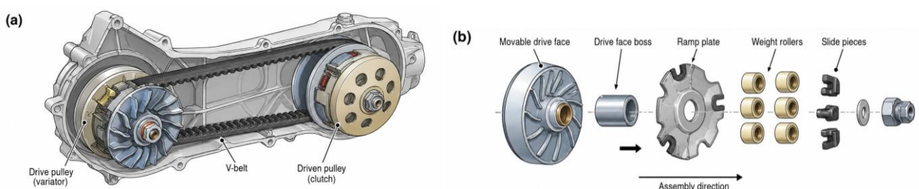
Figure 1. Motorcycle CVT system and weight-roller assembly: (a) CVT drive system and (b) exploded view of the variator and weight rollers.
