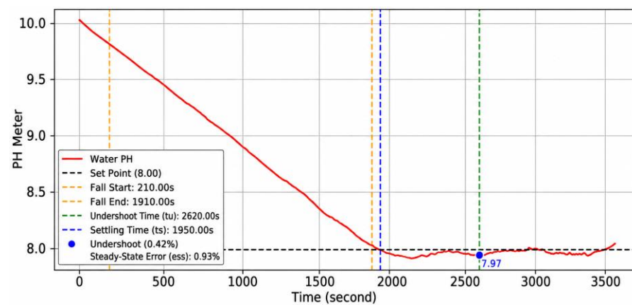
Figure 7. Second test result of pH control system response.
