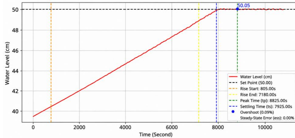
Figure 8. First test result of water level system response.
