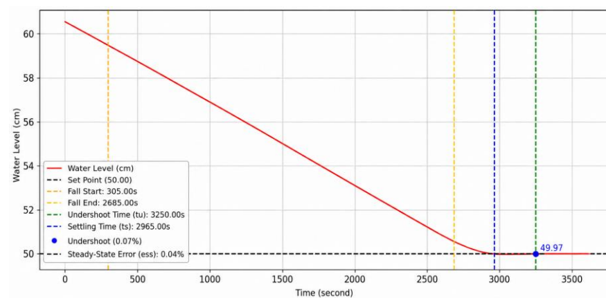
Figure 11. Second test result of draining system response
