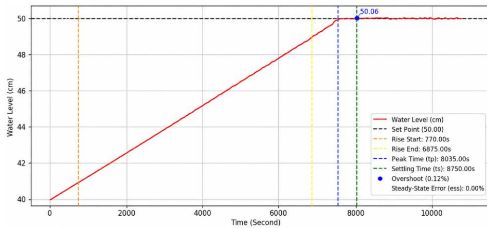
Figure 9. Second test result of water level system response.
