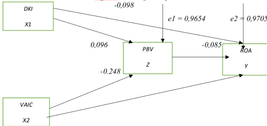
Figure 3 Path Diagram Equation Model
