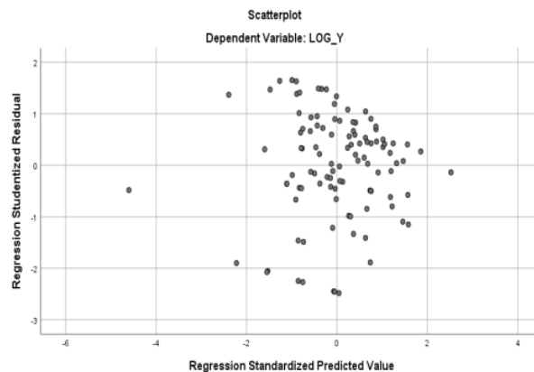
Figure 2 Heteroscedasticity Test
