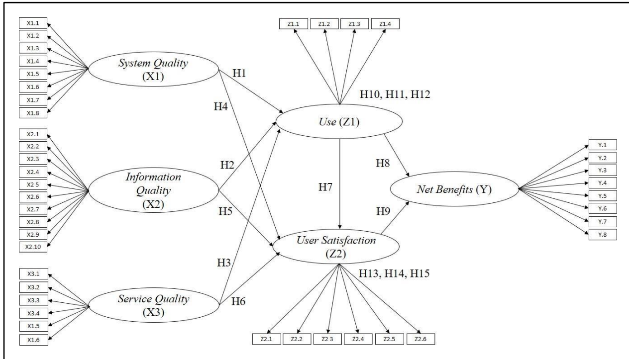
Gambar 1. Model Penelitian
