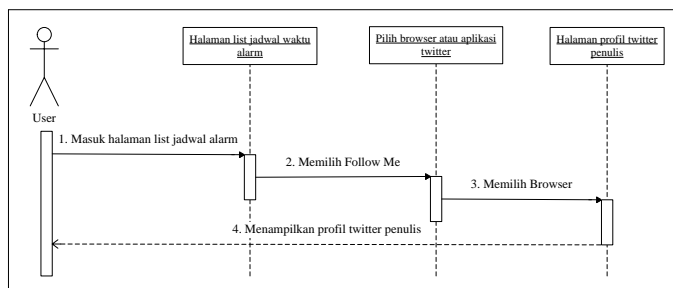
Gambar 11. Sequence Diagram Follow Me
