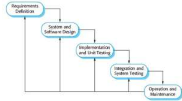
Gambar 2. Metodologi Waterfall [10]
