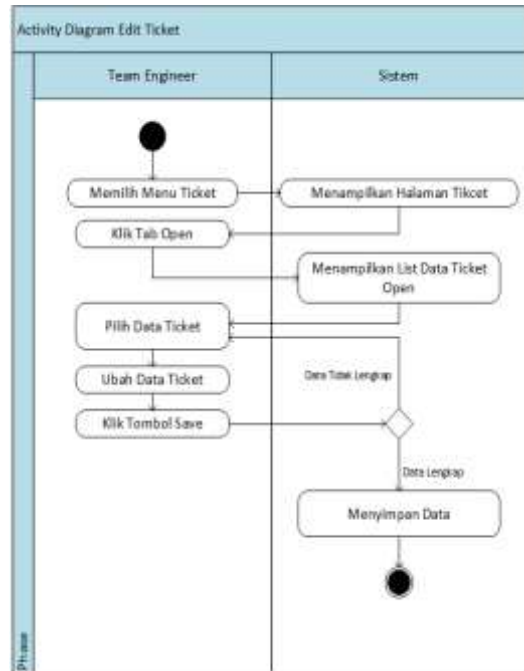
Gambar 5 Activity Diagram Edit Ticket
