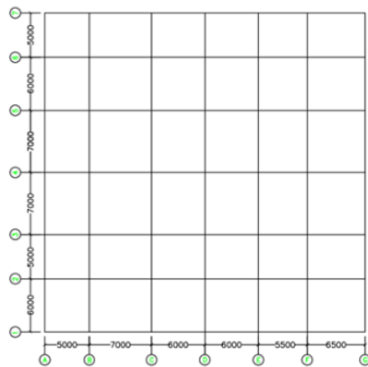
Figure 7. Model A Plan
