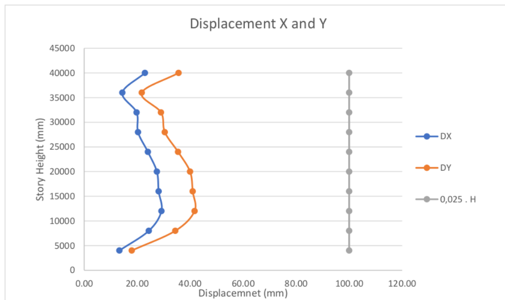
Figure 10. Model B Displacement
