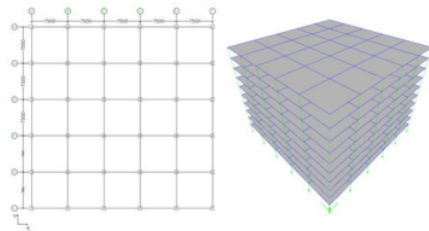
Figure 3. Regular Structure Model A Plan
