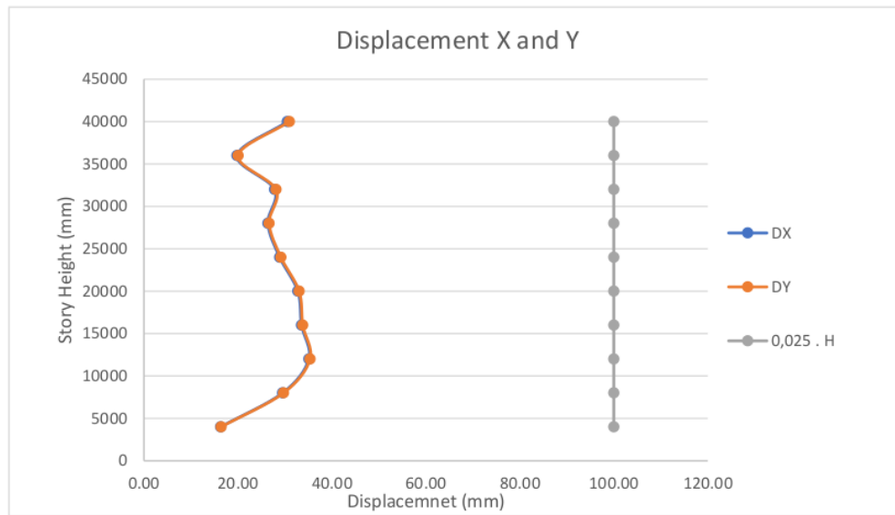
Figure 9. Model A Displacement
