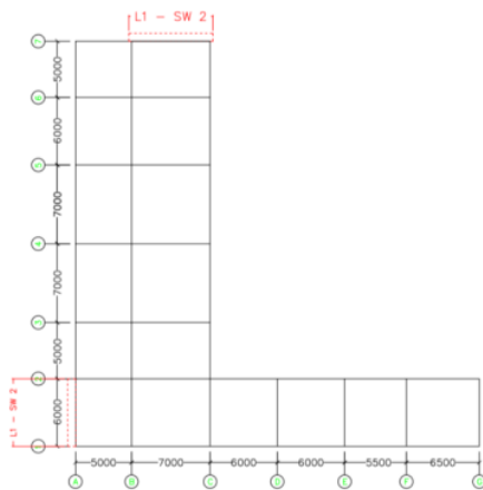
Figure 13. Modeling B SW-A
