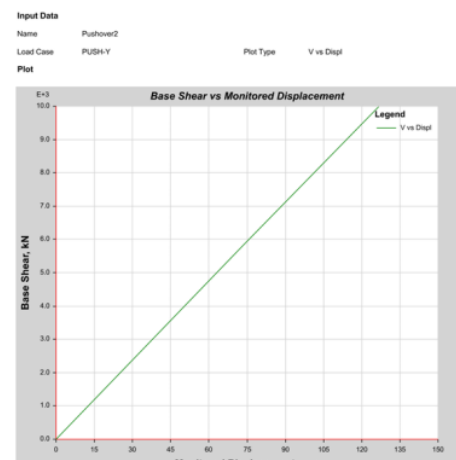
Figure 17. Base Shear vs Monitored Displacement PUSH X & PUSH Y model B SW-A
