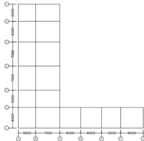
Figure 8. Model B Plan
