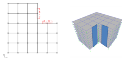
Figure 5. Model B Shear Wall Modeling Plan SW-1
