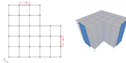
Figure 6. Model B Shear Wall Modeling Plan SW-2
