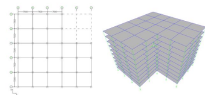
Figure 4. Irregular Structure Model B Plan
