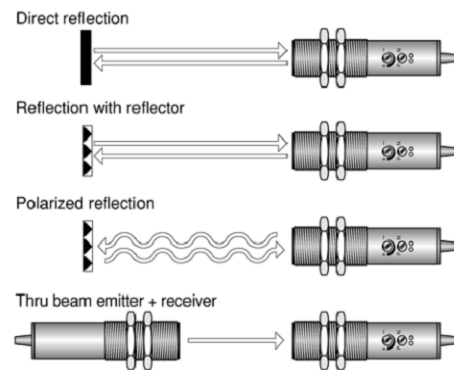
Gambar 5 Jenis Photo Electric Sensor
