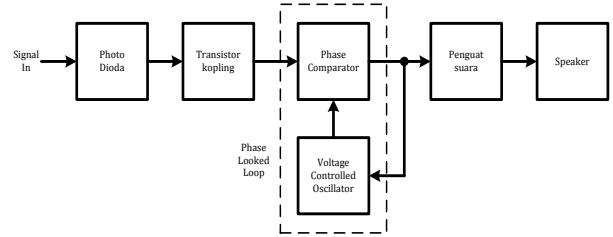
Gambar 3.3 blok diagram penerima audio
