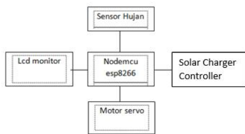
Gambar 1. Diagram Blok
