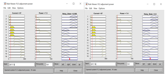
Gambar 18. Simulasi Matlab Fuzzy Logic Beban Laptop
