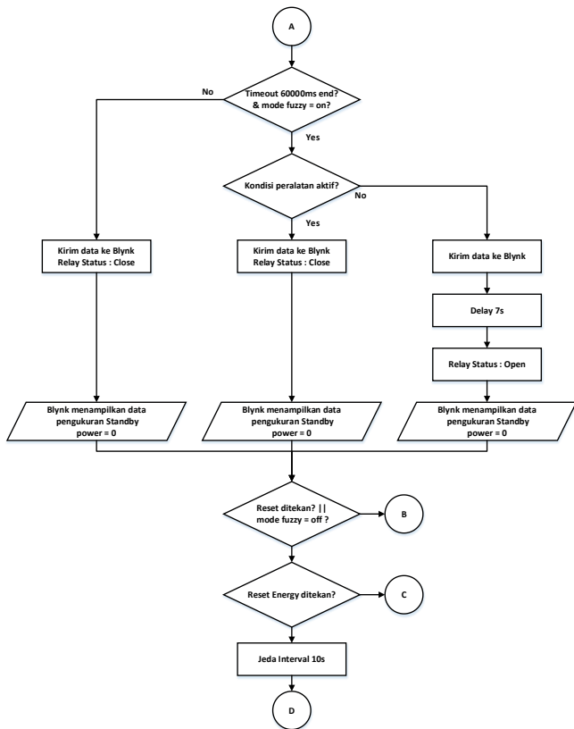
Gambar 4. Flowchart program
