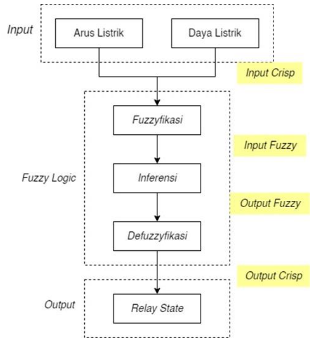
Gambar 5. Diagram Fuzzy Logic
