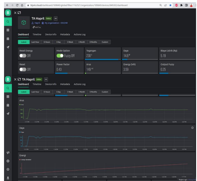
Gambar 10. Tampilan Dashboard Blynk Monitoring
