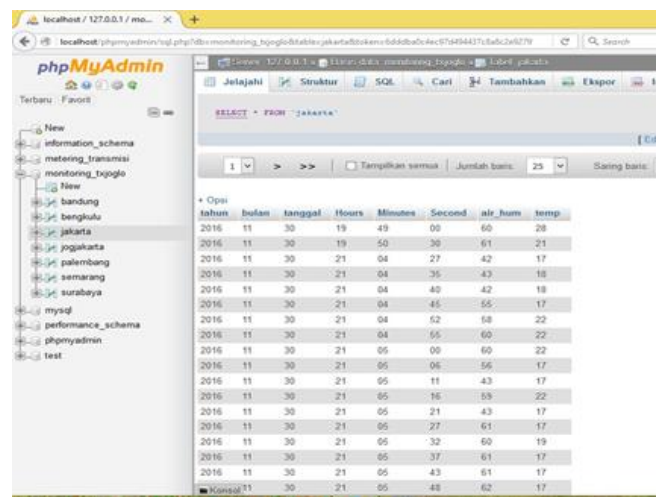
Gambar 6. Tampilan Database
