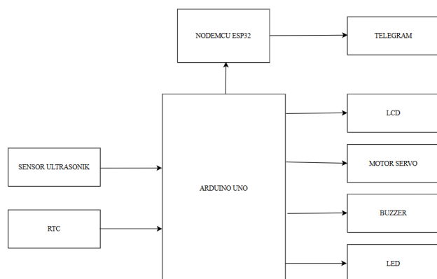
Gambar 1. Blok Diagram
