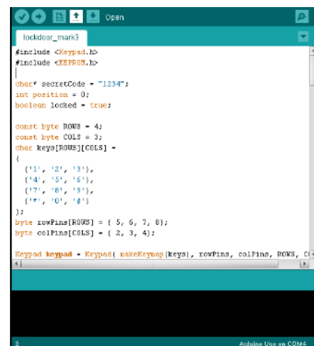
Gambar 15 program keypad IDE Arduino
