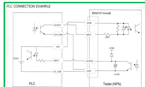
Gambar 4. Wiring Air Leak Tester
