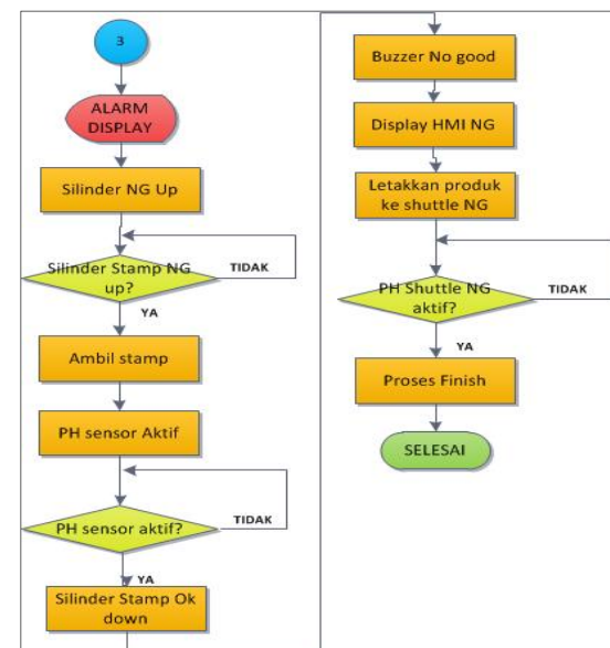
Gambar 9. Flow chart Program
