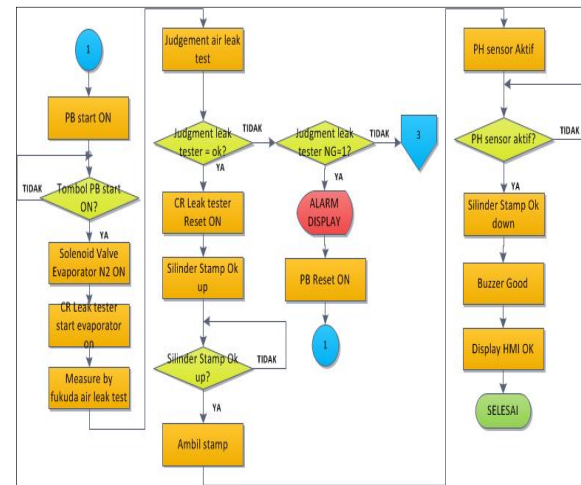
Gambar 8. Flow Proses Mesin Air Leak Test
