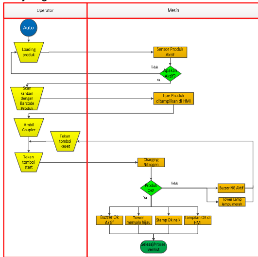
Gambar 8. Flow Proses Mesin Air Leak Test
