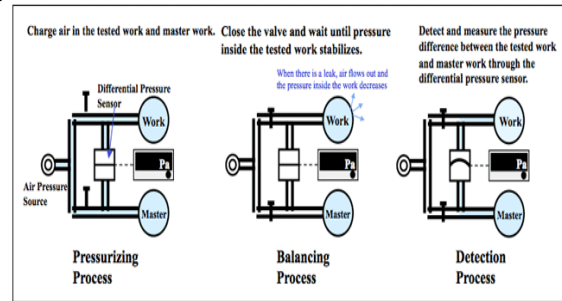
Gambar 1. Tahapan proses differential pressure air leak test
