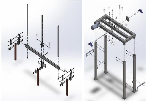
Gambar 3. Sistem knock down
