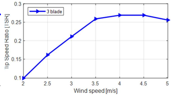
Figure 11. Tip Speed Curve Ratio to wind speed
