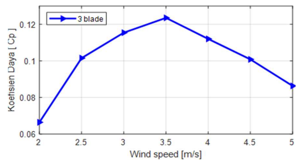
Figure 10. Power coefficient curve against wind speed
