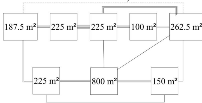
Gambar 10 Block Layout
