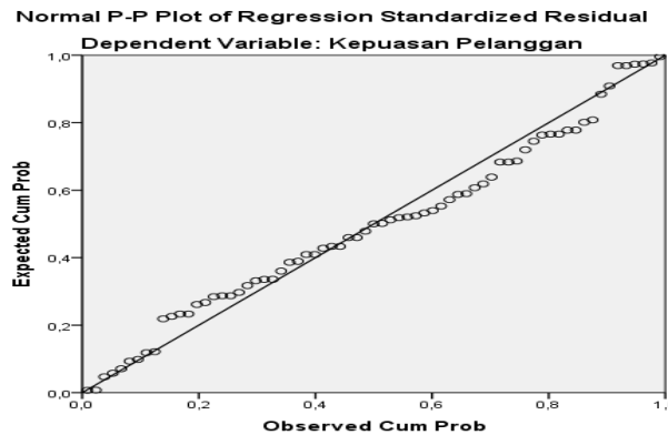
Gambar 4 Normal Probability Plot Sumber: Data diolah (2017)
