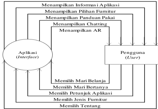
Gambar 4. Context Diagram
