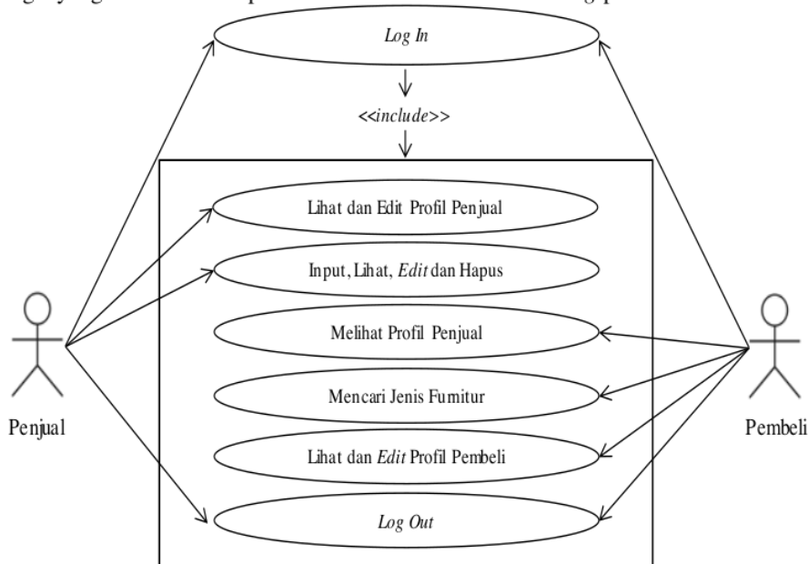
Gambar 3. Use Case Modeling
