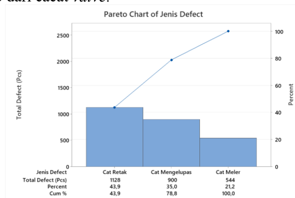
Gambar 5. Diagram Pareto Valve
