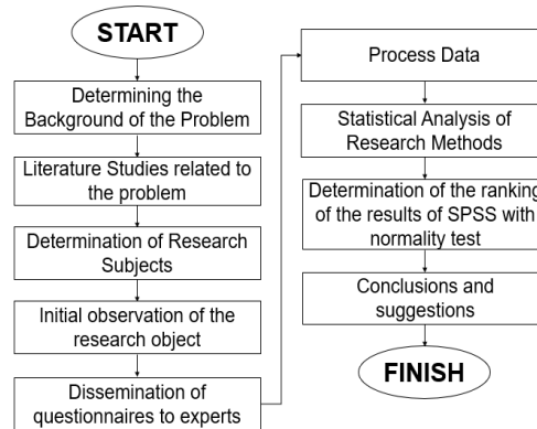
Figure 5. Research Flow
