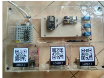
Figure 3. Implementation of Device System
