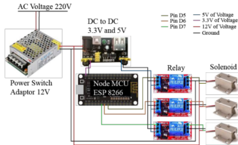
Figure 1. Design of Device System
