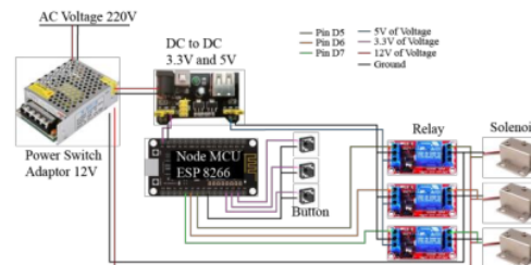
Figure 2. Design of circuit device for measure delay's value
