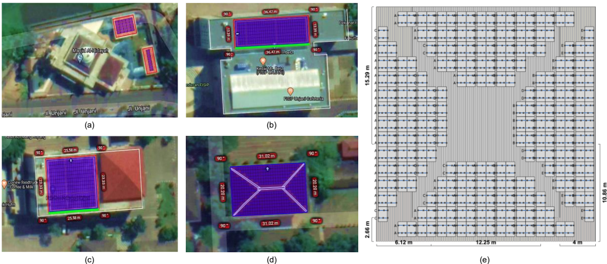
Figure 4. Simulation Rooftop PV using K2 Base; a) Al-Hidayah Mosque (AM), b) Faculty of Social and Political Science (FSPS), c) Faculty of Psychology (FPSI), d) Department of Electrical Engineering (EED) and e) base rail of Electrical Engineering Lab. (EEL)
