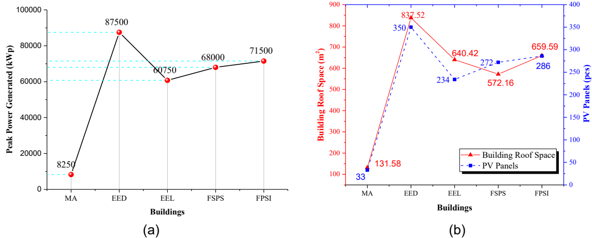
Figure 7. Simulation Result; a) Peak Power (kWp) Generated, b) Roof Area of a Building vs. Number of PV Panels
