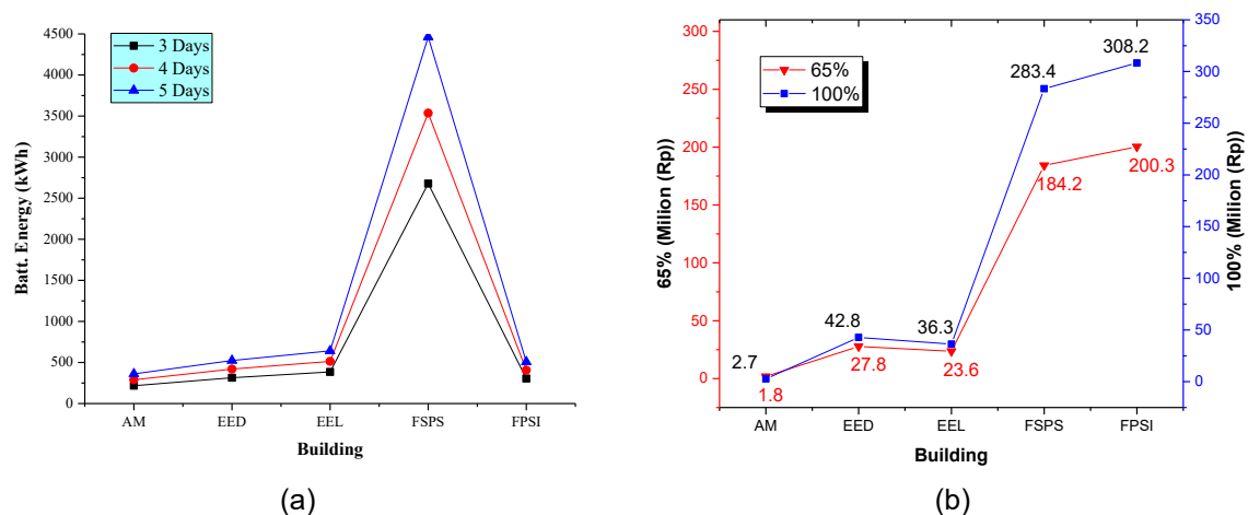
Figure 8. a) Battery Energy in kWh for each Building, b) Comparison of Feed in Tariff Export to the Grid
