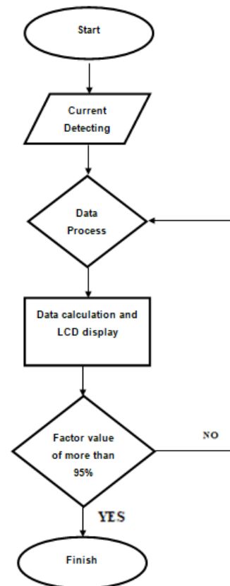
Figure 6. Flowchart of the system
