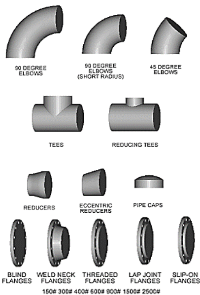
Gambar 1. Fitting (Sularso, 2006)
